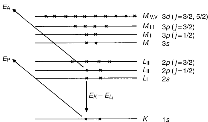
Figure 8.23 Illustration of a KL_1L_{II} Auger process
