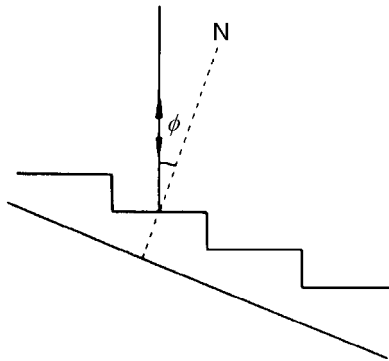
Figure 3.6 Use of a blazed grating at the blaze angle \phi ; N is the normal to the grating surface
