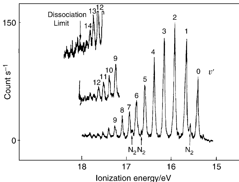
Figure 8.7 The He I ultraviolet photoelectron spectrum of \text{H}_2 . (Reproduced from Turner, D. W., Baker, C., Baker, A. D. and Brundle, C. R., Molecular Photoelectron Spectroscopy , p. 44, John Wiley, London, 1970)
