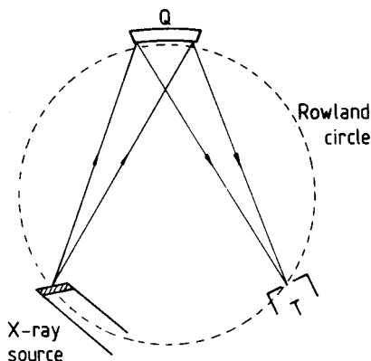
Figure 8.3 An X-ray monochromator using a bent quartz crystal Q; T is the target chamber
