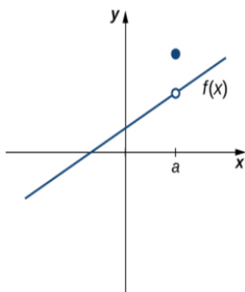
Figure 3. The function f(x) is not continuous at a because \lim_{x \rightarrow a} f(x) \neq f(a)
