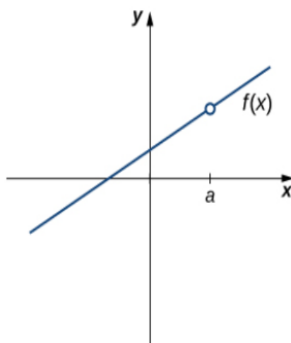
Figure 1. The function f(x) is not continuous at \mathbf{a} because f(\mathbf{a}) is undefined.
