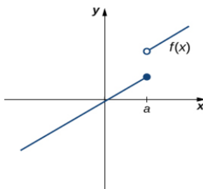
Figure 2. The function f(x) is not continuous at a because \lim_{x \rightarrow a} f(x) does not exist.
