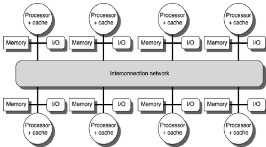
Distributed-memory multiprocessor
